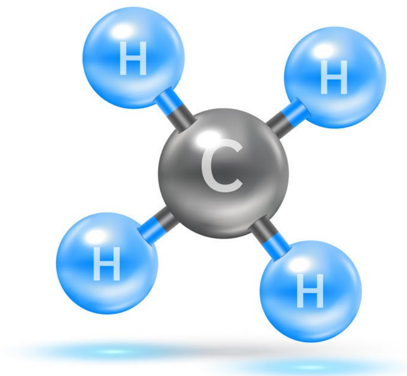
METHANE CH 4
