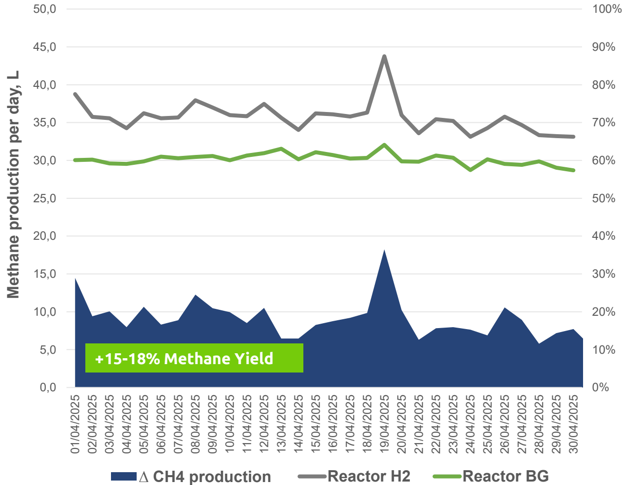
Results of laboratory studies of hydrogen biomethanation
