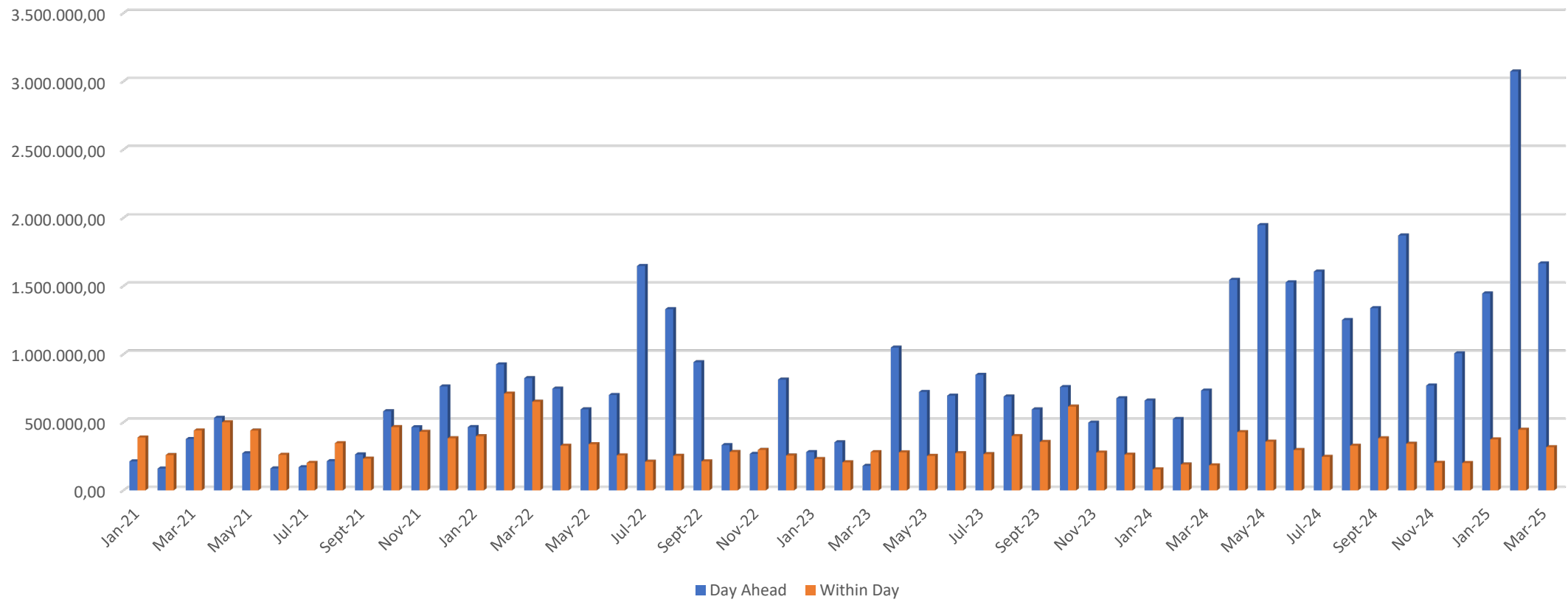
Evolution of Day Ahead and Within Day volumes (MWh)
