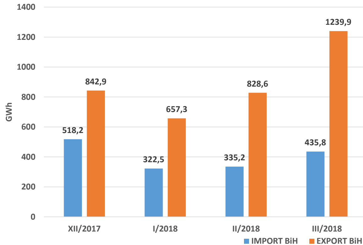
Scheduled Power Exchange – Winter 2017/2018
