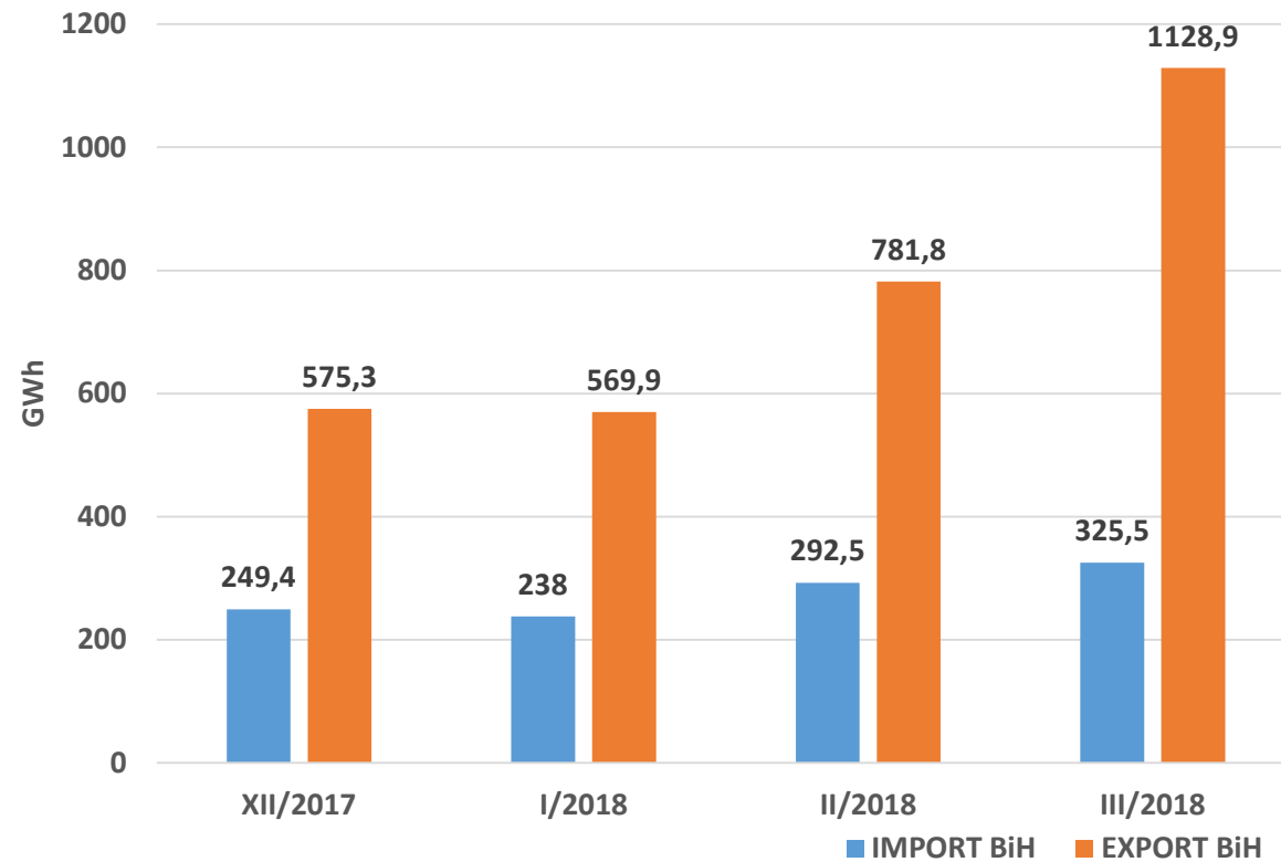
Real Power Exchange – Winter 2017/2018
